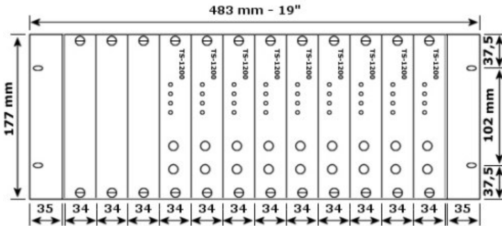
Vista Frontal
